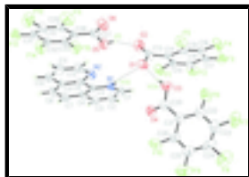
Fig. 1. The structure of (I). Displacement ellipsoids are drawn at the 30% probability level.
